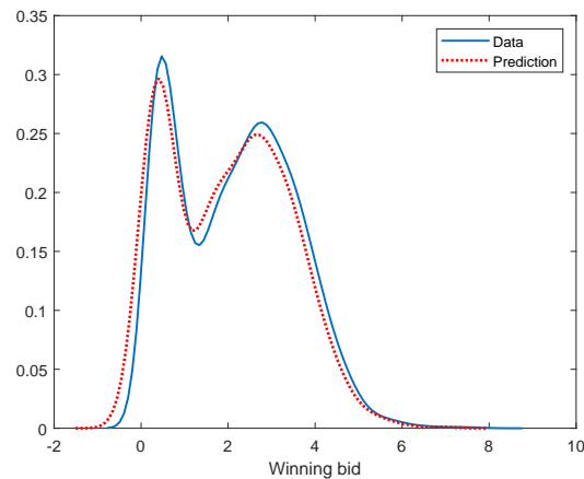
Figure 1: Simulated and Observed Winning Bids
