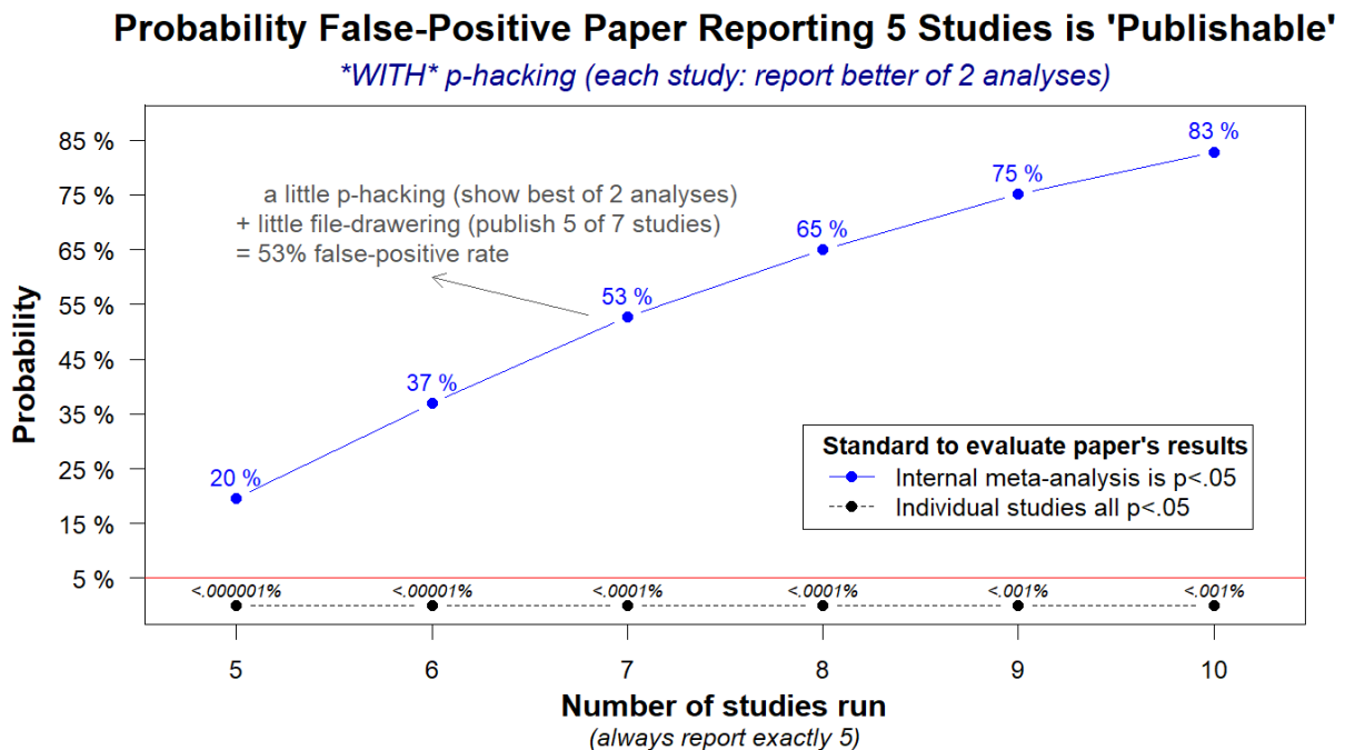
Fig 4. File-drawering + p-hacking and the probability of obtaining a false-positive five-study internal meta-analysis vs. five individual false-positive studies. The results were obtained by drawing the number of studies indicated in the x-axis (under the null). For each study, two separate independent t-values are drawn, and the higher one is kept (minimal p-hacking: two instead of one analysis attempted). The five studies with the larger t-values among these were converted onto Cohen's d, and aggregated via a random-effects meta-analysis. This was repeated 10,000 times. The top line depicts the percentage of simulations where the overall meta-analysis obtained p < .05 , and the bottom one where all five of the selectively reported studies would be expected to be significant, based on the binomial distribution. For example, the two left-most dots show that when the 5 studies reported are the only ones attempted, and for each, the best of two independent analysis run is reported, there is a 20% chance that the internal meta-analysis will be p < .05 , and only 1 in a 100 million chance that the five studies will be individually significant. R Code to reproduce figure: https://osf.io/pdyhv/ .
