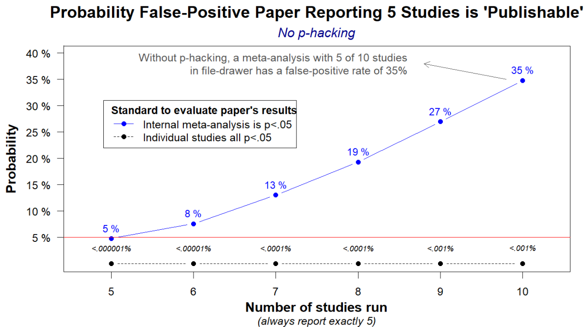
Fig 3. File-drawing and the probability of obtaining a false-positive five-study internal meta-analysis vs. five individual false-positive studies. The results were obtained by drawing the number of studies indicated on the x-axis under the null, generating individual t-values for those individual studies, and keeping the five largest t-values that were generated. Those five t-values were then converted into Cohen's ds, and aggregated using random effects meta-analysis. This was repeated 10,000 times for each of the 5, 6, 7, 8, 9, and 10 total t-values. The y-axis depicts the percentage of simulations for which the overall meta-analysis obtained p < .05 , and for which all five of the studies were individually significant. For example, the two right-most dots show that when 10 studies are attempted, and the best 5 are reported, there is a 35% chance that the internal meta-analysis will be p < .05 , but there is less than a 1/10,000 chance that the five studies will be individually significant. R Code to reproduce figure: https://osf.io/pdyhv/ .
