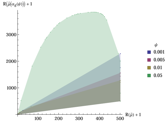
Figure 6: A high spending rate \psi potentially exhausts the wealth of a geometric testimator and produces excessive risks. These results are for p = 500 tests and rates \psi = 0.001, 0.005, 0.01, \text{ and } 0.05 .
