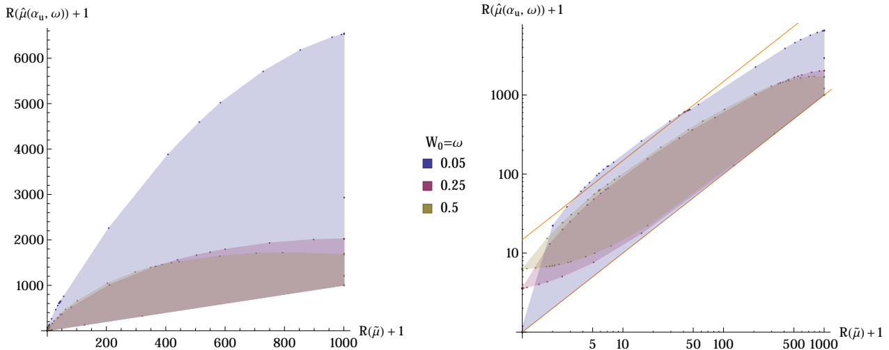
Figure 5: Varying the initial wealth and payout influence the feasible set of risks that contrast the risk inflation oracle to the universal estimator \hat{\mu}(\alpha_u(\cdot), W_0, \omega) . The initial wealth varies over W_0 = 0.05, 0.25, and 0.50 with p=1,000 tests on the scale of risks (left) or log risks (right).
