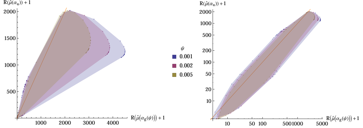
Figure 7: The universal alpha investing testimator \hat{\mu}(\alpha_u(\cdot), W_0, \omega) (y-axis) produces typically smaller risks than geometric testimators \hat{\mu}(\alpha_g(\cdot), W_0, \omega) (x-axis). The geometric rates are \psi = 0.001, 0.002, \text{ and } 0.005 with p = 1,000 .
