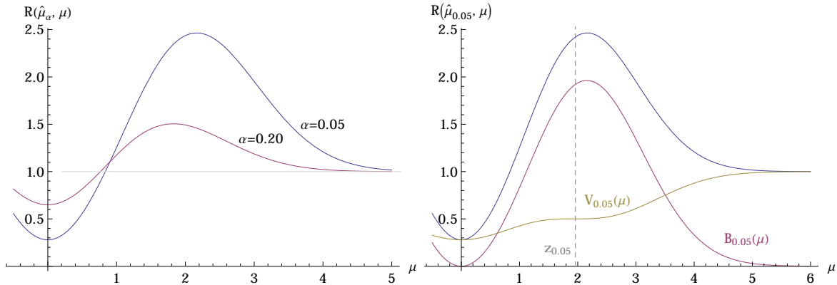
Figure 2: The risk of testimators peaks near z_\alpha due to a large contribution from the bias as the level \alpha decreases. (a) Risk of testimators with \alpha = 0.05, 0.20 versus \mu . (b) Squared bias and variance components of the risk of \hat{\mu}_{0.05} .
