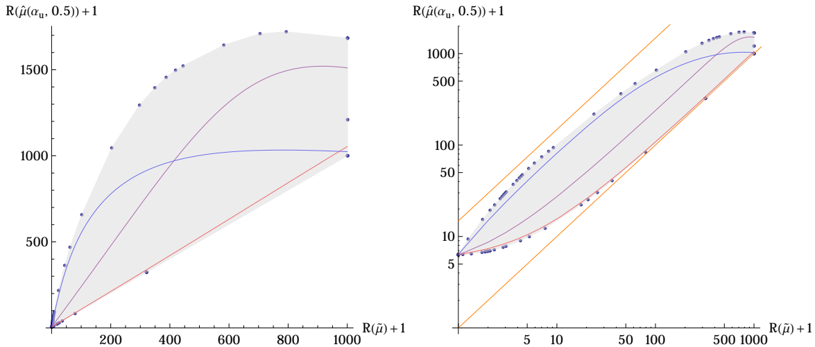
Figure 3: The shaded feasible set identifies the possible risks of the oracle estimator \tilde{\mu} and universal estimator \hat{\mu}(\alpha_u(\cdot), W_0, \omega) with W_0 = \omega = 0.5 , p=1,000 . The left frame emphasizes models with substantial signal; the right frame (log scale) highlights nearly black models. Curves within the feasible set show the risks as the signal levels varies in the model (20). Boundary points show calculation locations described in Section 5; the line parallel to the diagonal in the right frame is the risk-inflation boundary discussed in the text.
