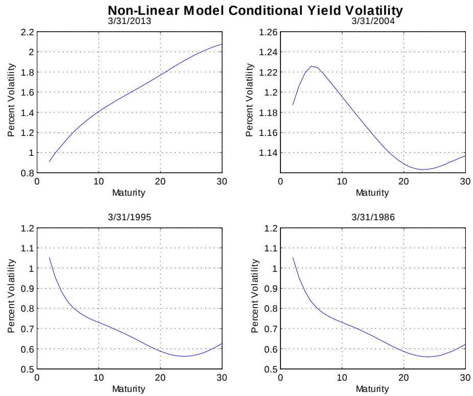
Figure 14: Conditional yield volatility of zero coupon bonds on four selected dates.
