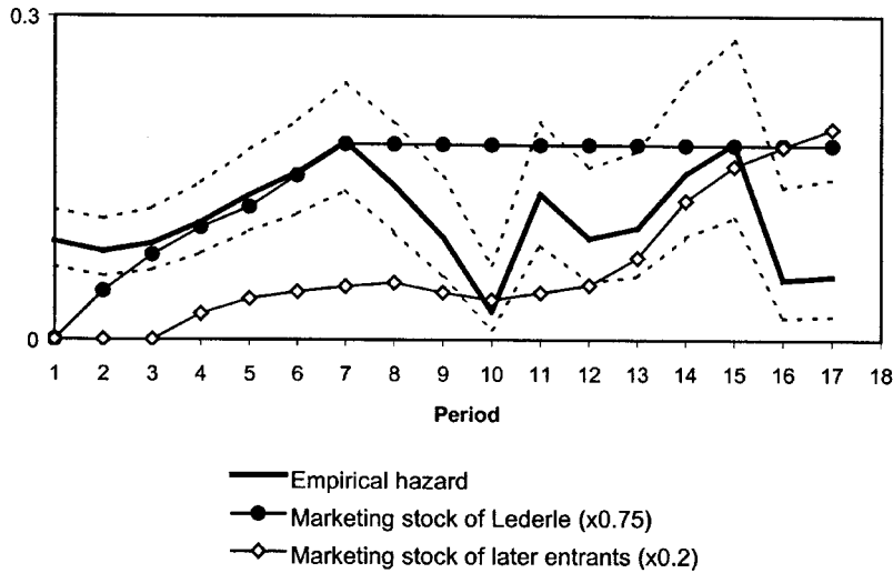
FIG. 2.—Empirical hazard rate and marketing stock. The broken lines around the empirical hazard rate indicate the SE interval (+/- 1). We computed SEs using a logit hazard model. The interval is not symmetric because the logit model is linear in the log odds of the hazard rate, not in the hazard rate itself.
